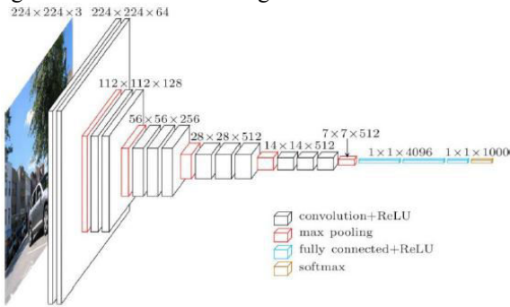
Fig 2 – VGG16 architecture
